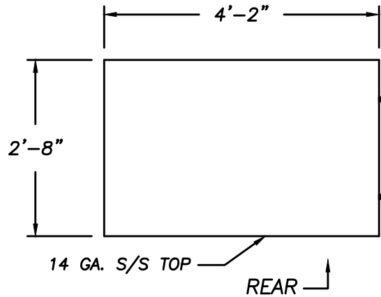
PLAN VIEW 1/2"=1'-0"
