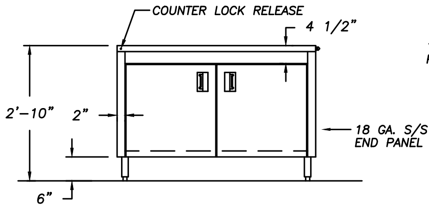
REAR ELEVATION 1/2"=1'-0"
